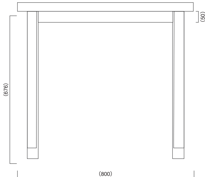
[側面]
