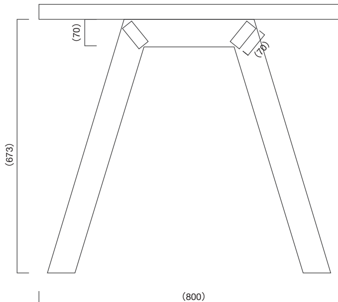
[側面]
